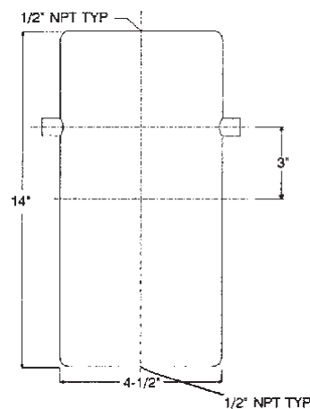
4" Catalog No.: CP-4-C-8-N
